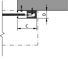
WANDMONTAGE
